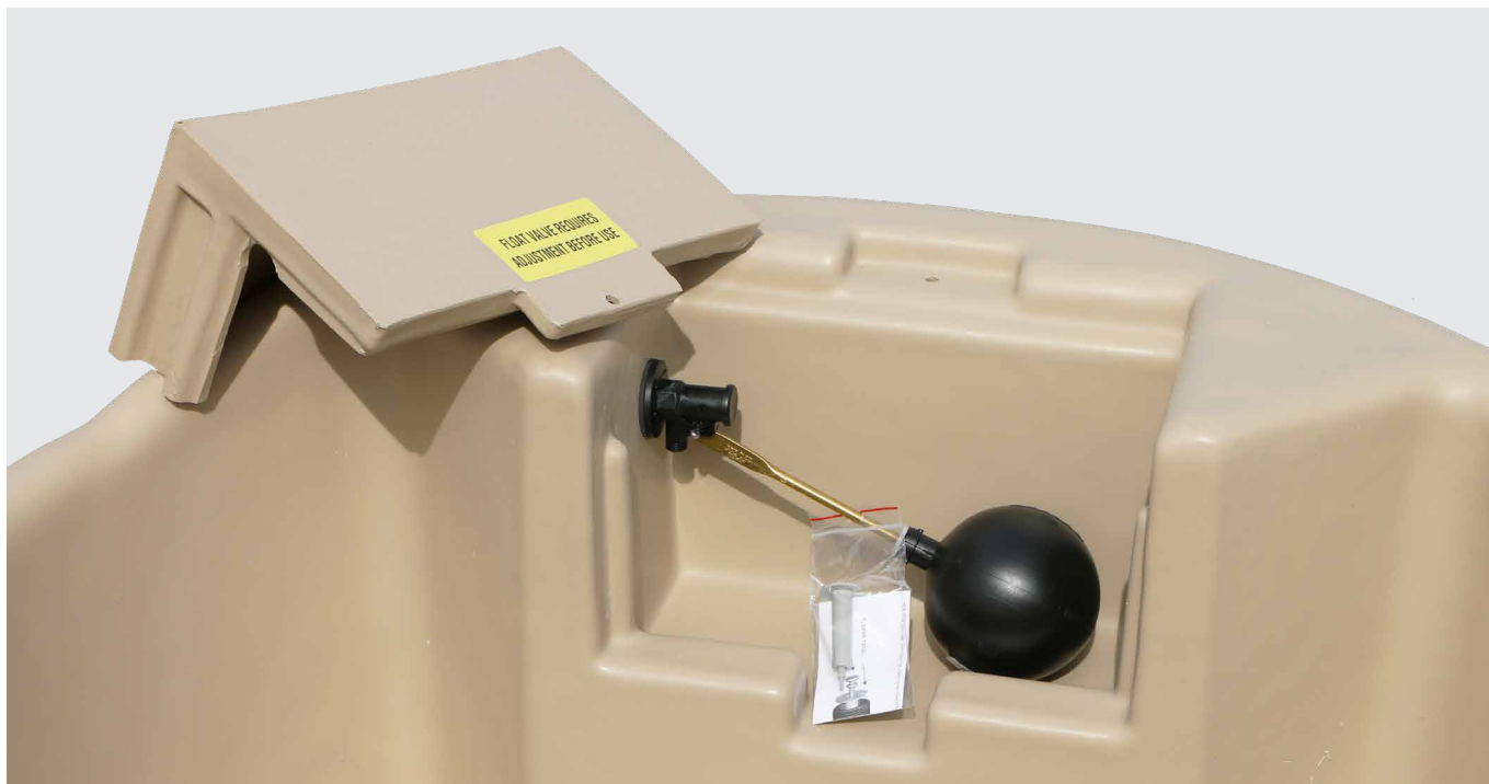
Float valve protected by slide up access cover
